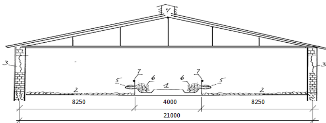
Fig. 1. Cross-section of a barn for 200 cows (21 m wide)
