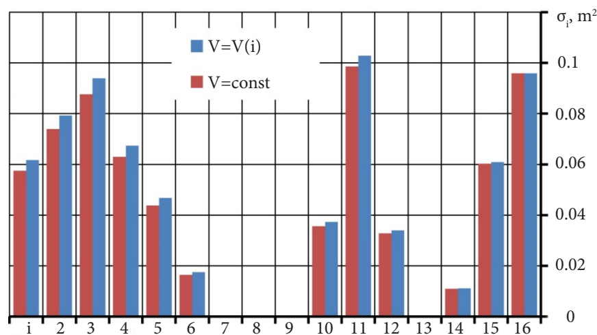
Figure 6. Velocity distribution V_i in the air intake pipes
