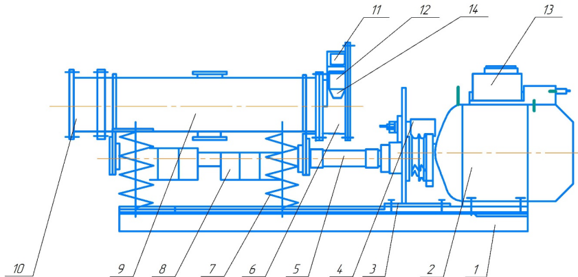
Figure 3. Constructive scheme of the experimental vibrating mill of continuous action MVE-5: 1 – frame; 2 – electric motor; 3 – V-belt transmission; 4 – riser; 5 – elastic cardan shaft; 6 – reloading chute; 7 – elastic supports; 8 – vibrating exciter; 9 – grinding chambers; 10 – transitional gutter; 11 – loading branch pipe; 12 – unloading tray; 13, 14 – control panels
