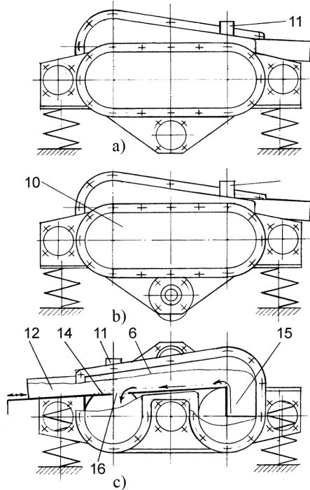
Figure 4. Scheme of regulation of supply of loading of a mill of MVE-5: 14 – sunroof; 15 – vertical gate; 16 – reloading window
