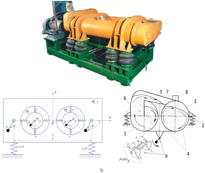
Figure 9. Vibrating mill MV-400: a) general view of industrial model; b) kinematic scheme
