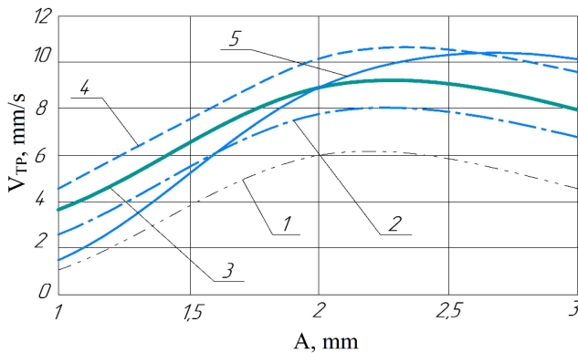
Figure 8. Graph of the dependence of the transport velocity V_{TP} on the amplitude A at the optimal frequency \omega value for different bulk materials: 1 – cherry stones; 2 – polystyrene granules; 3 – peas; 4 – ceramic balls, 5 – steel balls
