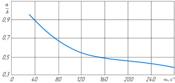
Figure 1. Dependence of the coefficient \frac{a}{A} on the frequency of oscillations
