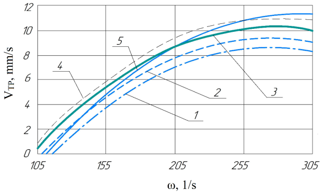
Figure 7. Graph of the dependence of the transport velocity V_{TP} on the frequency \omega at the optimal value of the amplitude A for different bulk materials: 1 – cherry stones; 2 – polystyrene granules; 3 – peas; 4 – ceramic balls, 5 – steel balls
