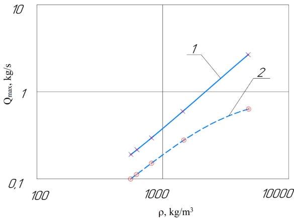
Figure 5. Dependence of maximum productivity Q_{max} on the density of bulk material \rho for different schemes of vibrating excitation: 1 – with a central location; 2 – with the lower location
