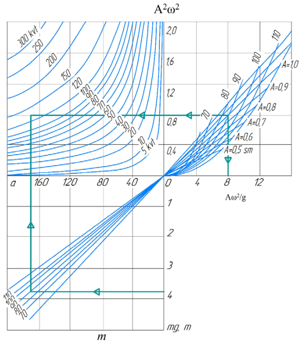
Figure 2. Nomogram for determining the power consumed for grinding
